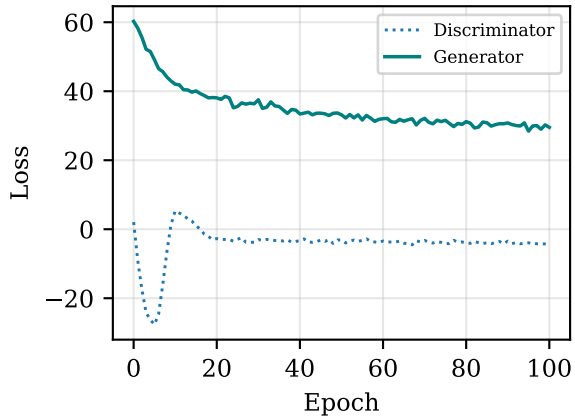
CIFAR-10
